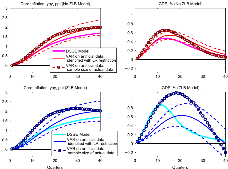
Fig. 11. Monte Carlo experiment.
